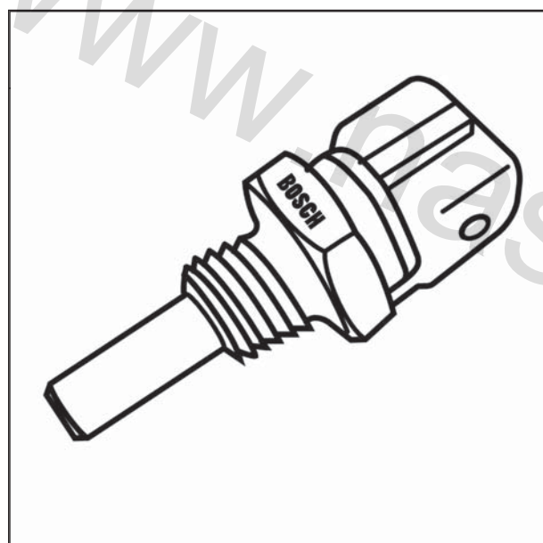
Engine- temperature -sensor 1 Electrical connection, 2 Housing, 3 NTC resistor
