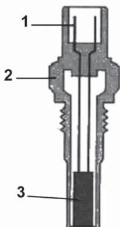
Engine- temperature -sensor 1 Electrical connection, 2 Housing, 3 NTC resistor
