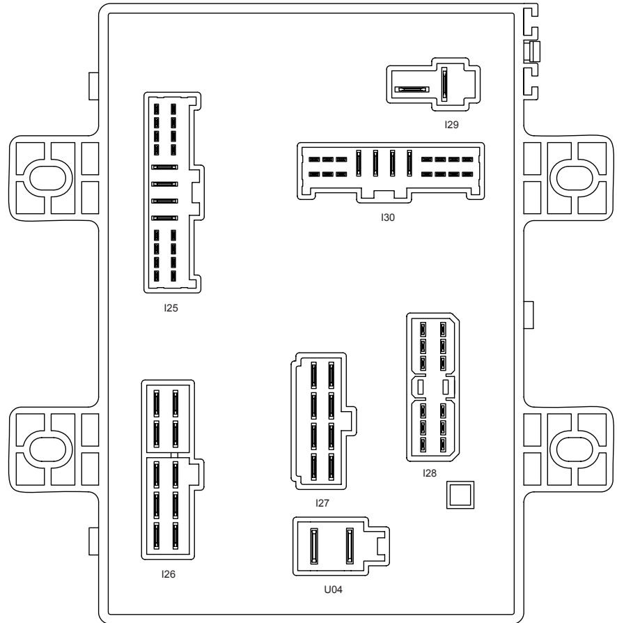
I/P Fuse and Relay Box Back View
