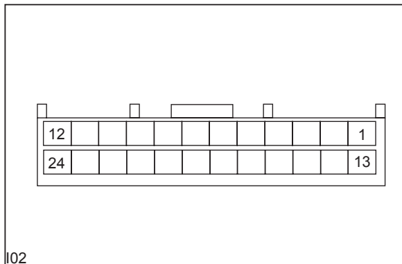
Instrument Cluster-2 Connector
