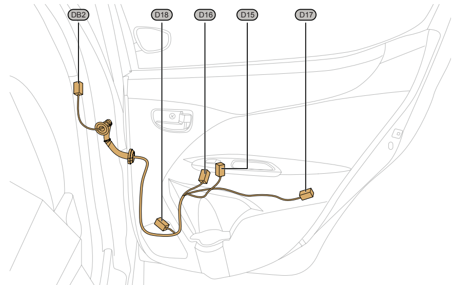
RR Door Harness
