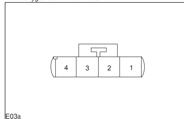
E03a Pin Definition
