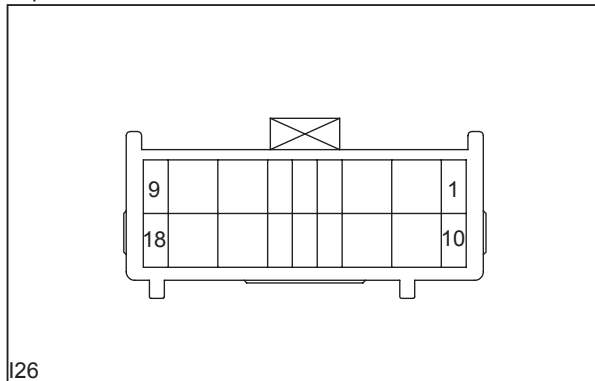
I26 Pin Definition
