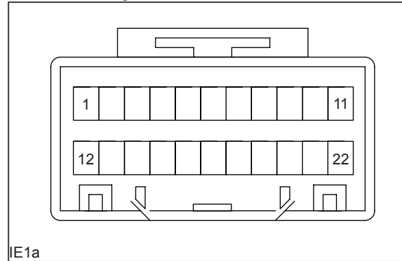
IE1a Pin Definition
