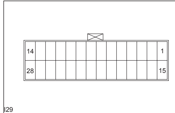
Instrument Cluster -2(W) Connector
