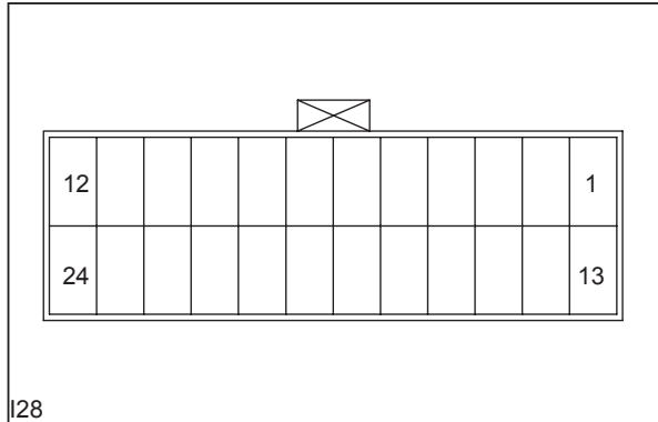
Instrument Cluster-2(B) Connector
