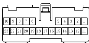
M15 A/C control panel A
